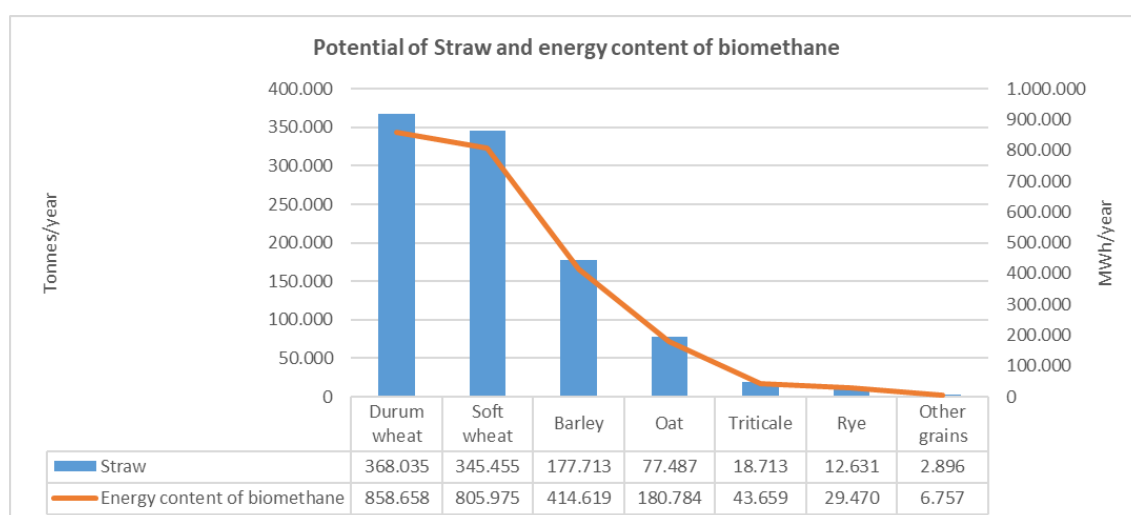
Figure 4-4. Potential and energy content of biomethane from straw.
