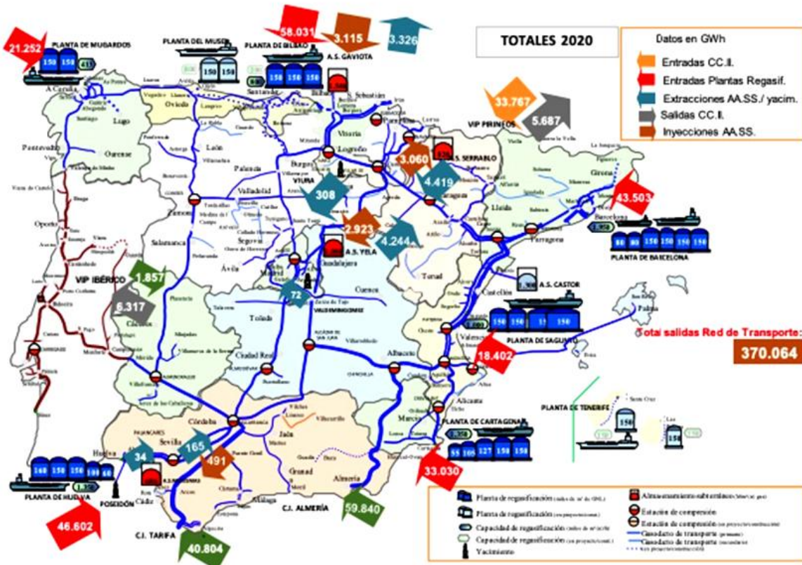
Figure 7-6. Natural gas grid in Spain
