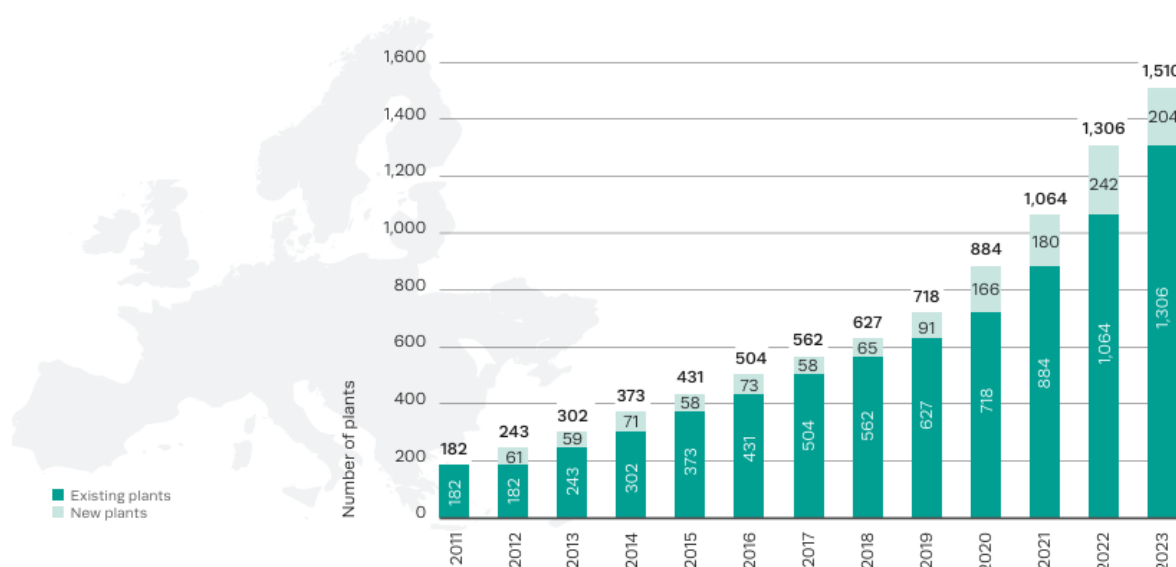
Figure 1-1. Development of the number of biomethane plants in Europe Error! Bookmark not defined.
