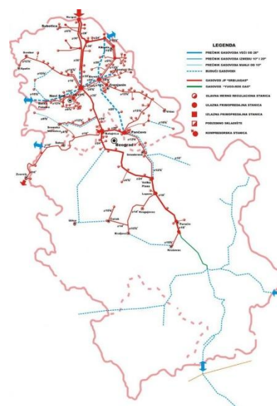
Figure 8-4. Map of the natural gas pipeline in Serbia
