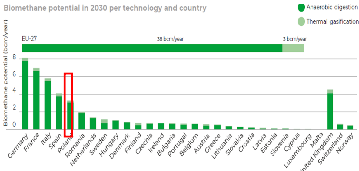
Figure 6-2. Biomethane potential in 2030 in Poland (Gas for Climate report 2022)
