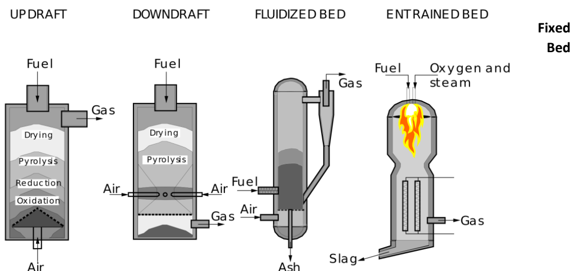
Figure 11 Types of gasifiers, Image Source : H24U
