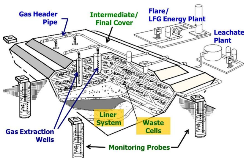
Figure 9 Landfill Gas Extraction Process.
