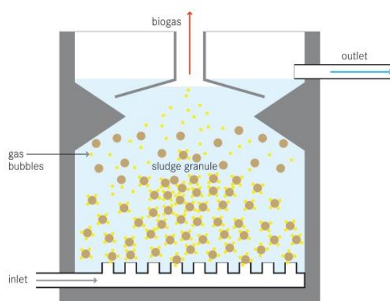
Figure 8 Upflow Anaerobic Reactor Sludge Blanket digestion, UASB
