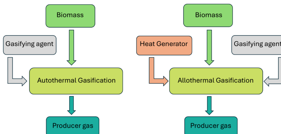
Figure 10 Different heat application for gasification processes. Source : EBA
