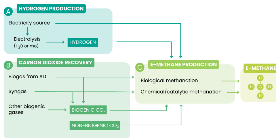
Figure 13 Methanation production process. Source : EBA 13
