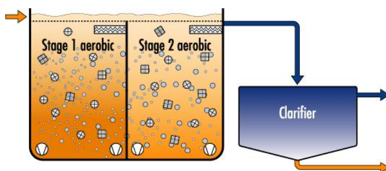
Figure 7 Biofilm reactor system. Image source: Lenntech
